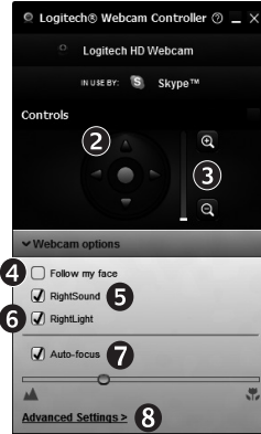
Webcam Controller
